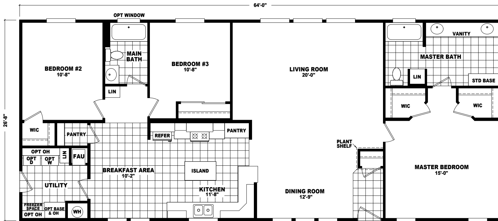
MODEL: DN-2864A APPROXIMATELY 1706 SQ. FT. 3 BEDROOM, 2 BATH
